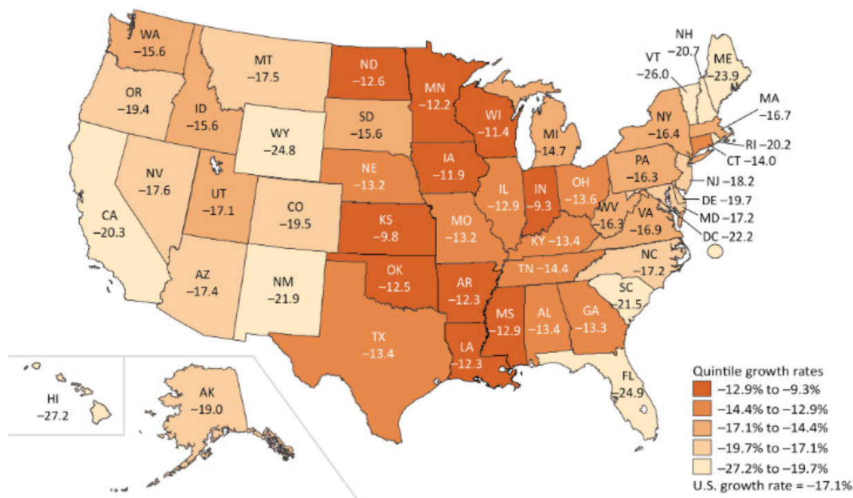
Figure 2: Percent Change in Outdoor Recreation Employment, 2020, reproduced from the BEA 15
